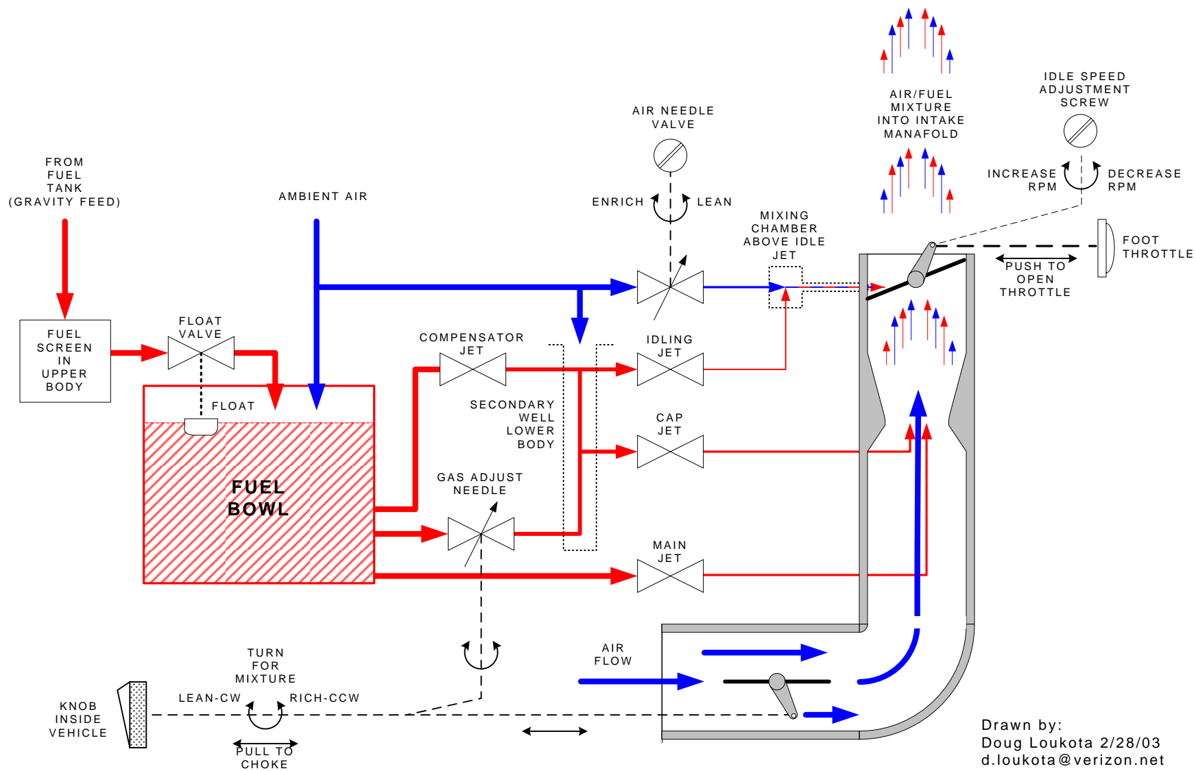
Single Venturi Zenith Carburetor Flow Diagram
